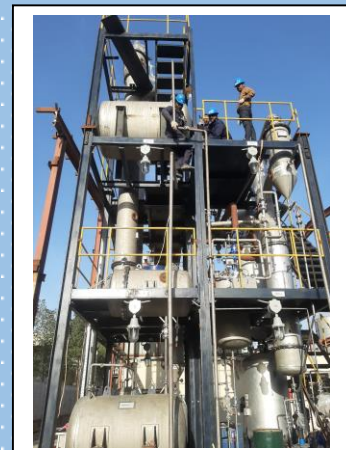
Liquid-Liquid Extraction
